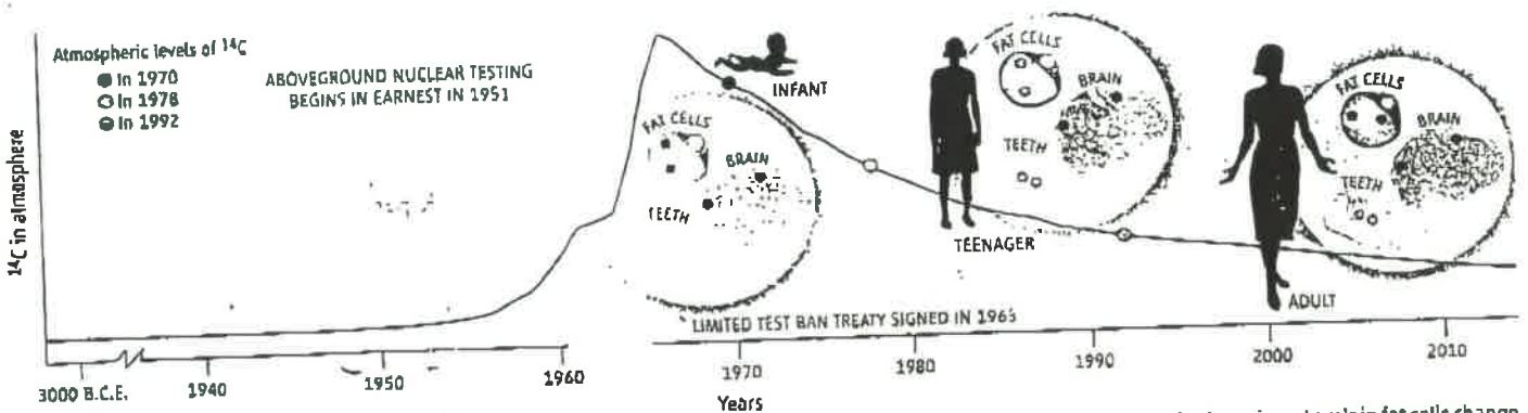
Atomic child. 14 C levels in DNA from visual and memory neurons stay the same throughout life, indicating no neurogenesis in these brain regions. Levels in fat cells change, suggesting constant fat cell turnover. 14 C levels in tooth enamel remain constant and can be used to calculate a person's birth date.
